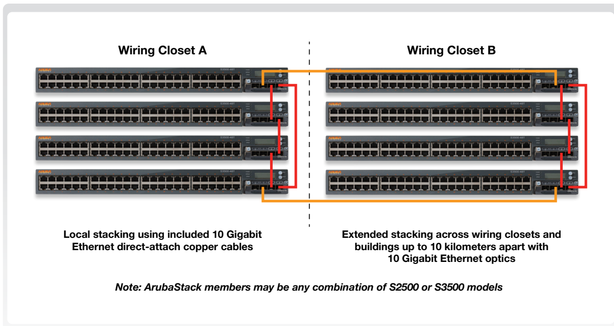
Figure 2. ArubaStack options
